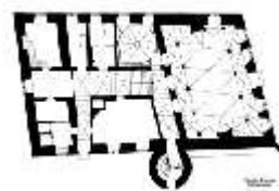
CoR.IV, Grundriss, Erdgeschoss, DE002516, BSV
